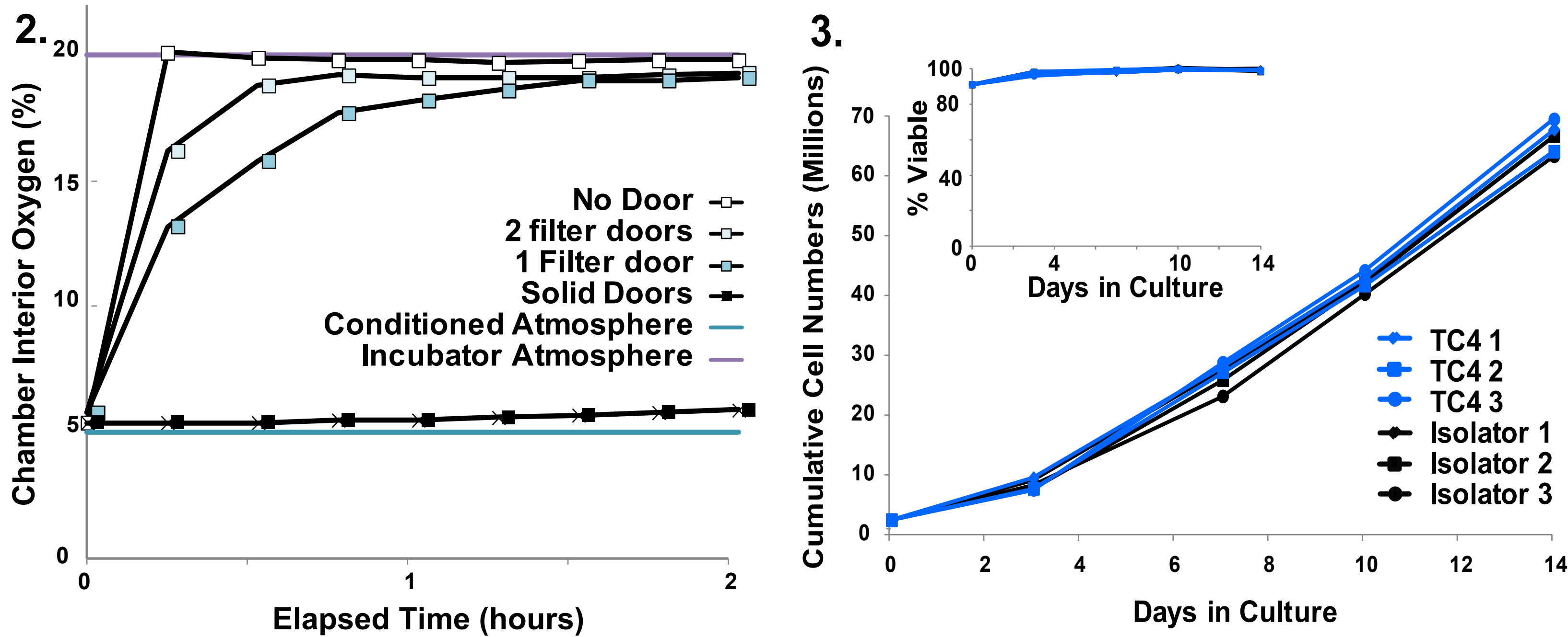
Figure 2. Equilibration with Incubator Air An oxygen probe was sealed into a test TC4 chamber through a small hole in the top surface. The chamber was equilibrated in the barrier isolator to 5% oxygen to assess equilibration with incubation air (~20% oxygen). The test chamber was assayed three times in each configuration; with no doors, with two covers in place over the filters, with one filter uncovered, and with two filters uncovered. Interior oxygen levels in the chamber were recorded every fifteen minutes. With filter doors uncovered on each end, the chamber equilibrated rapidly, reaching maximal O 2 in about 30 min. The mean of the values for three trials is shown for each configuration.
